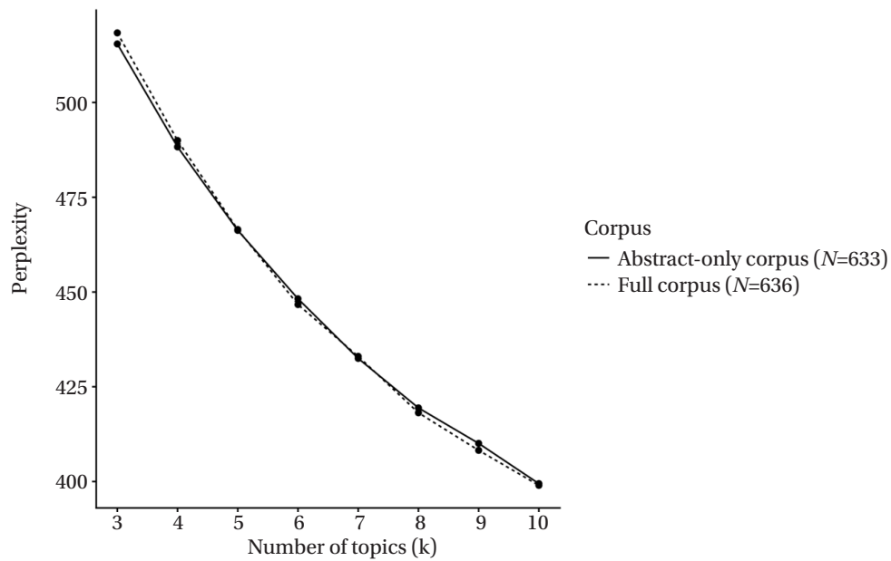
Supplementary Figure 3. Perplexity across candidate latent Dirichlet allocation models ( k=3-10 ) in the effective full corpus ( N=636 ) and abstract-only sensitivity corpus ( N=633 ).
